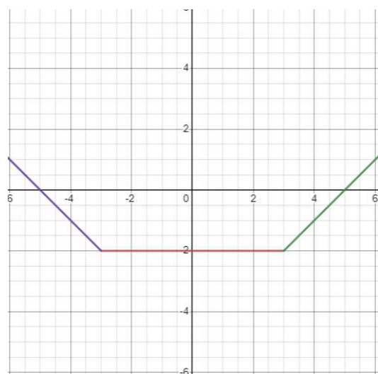
Piecewise function
