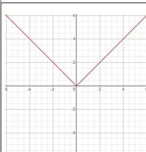
Absolute Value Function
