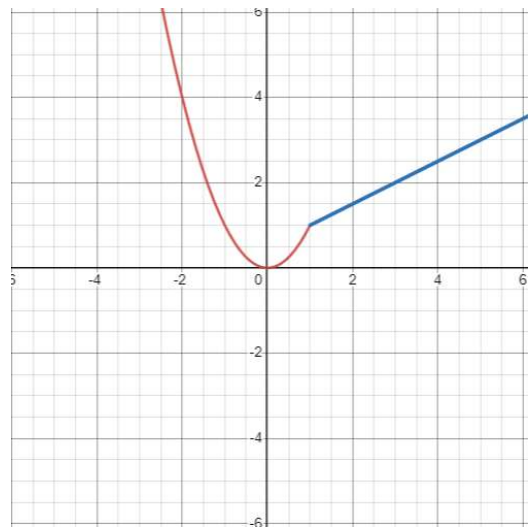
Piecewise function
