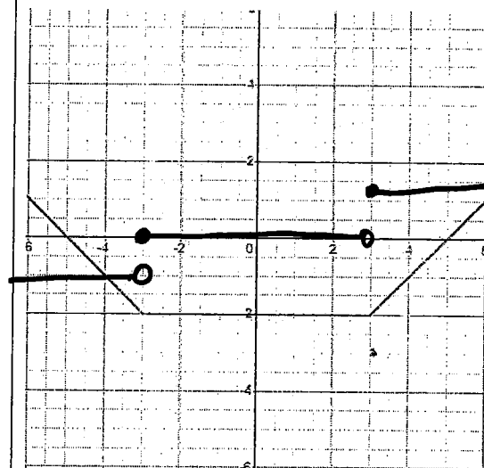
Piecewise function
