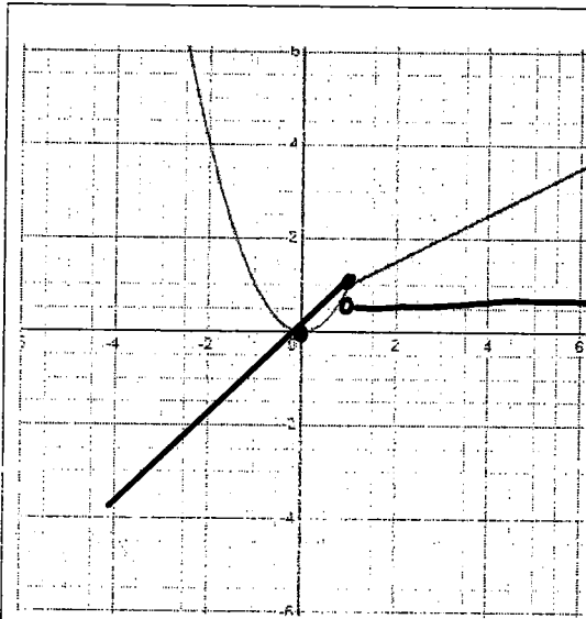
Piecewise function
